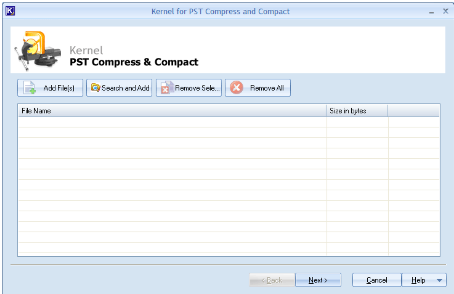
Figure 2.1 : Main Window
